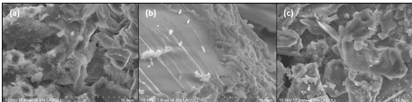
Microphotographies (SEM) of Mortar: a) CM, based on cement, (b) GM1, based on volcanic ash with NaOH and (c) GM2 based on volcanic ash with NaOH+Na 2 SiO 3 , Maria Vargas et al., pp. 148-159
